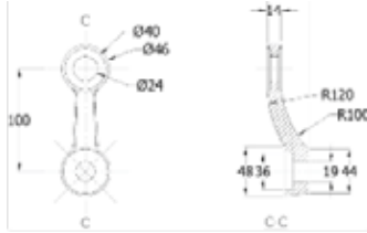
Lama Spider 4'lü Lama Spider 4
